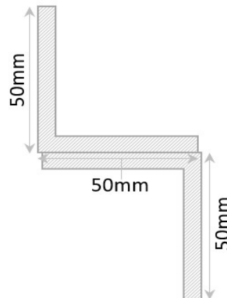
L Bracket
