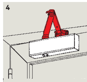
Hold-open arm installation Adjustable for hold-open up to 150°.
