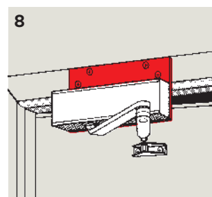
Drop plate installation For installation on frame (or door) when direct fixing of closer is not possible.
