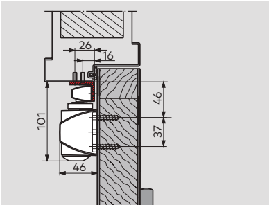
Angle bracket For push-side fixing of the slide channel to door frames with a deep reveal.
