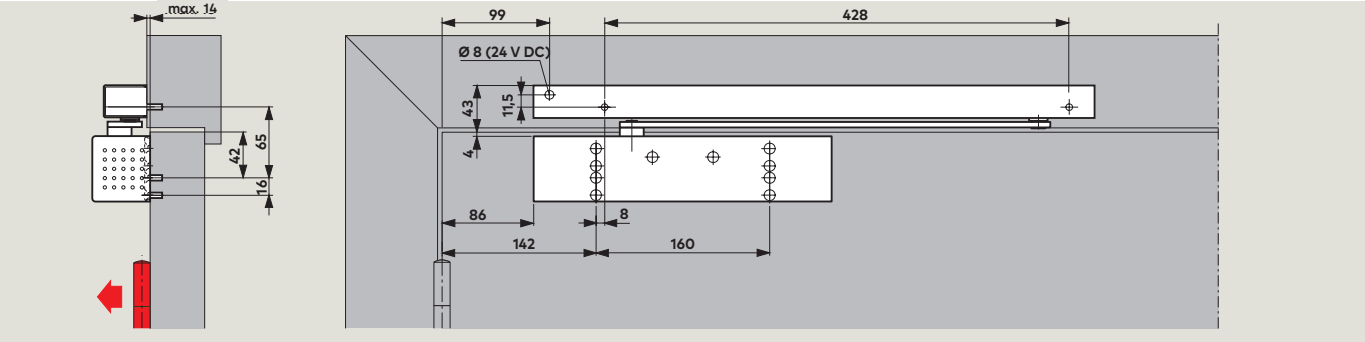
TS 92 B closer with G-EMF slide channel assembly, pull-side fixing Example: Anticlockwise-closing (ISO 6) door; mirrored arrangements apply to clockwise-closing (ISO 5) doors.
