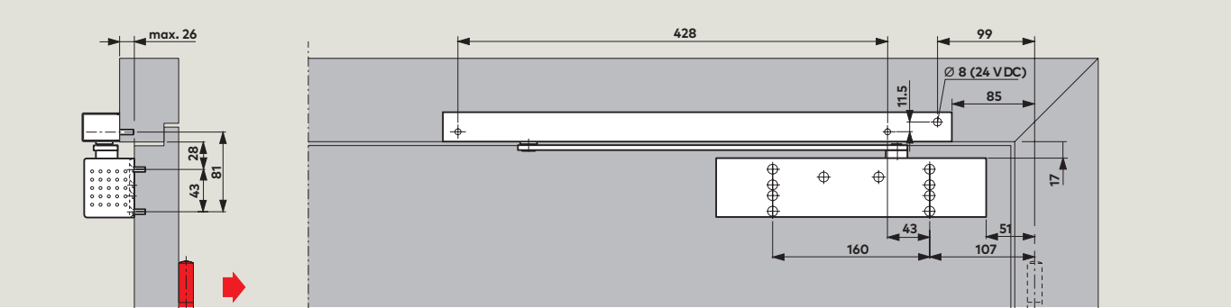
TS 92 G closer with G-EMF slide channel assembly, push-side fixing Example: Anticlockwise-closing (ISO 6) door; mirrored arrangements apply to clockwise-closing (ISO 5) doors.
