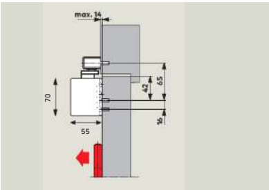
TS92B Door leaf fixing, pull side with cover
