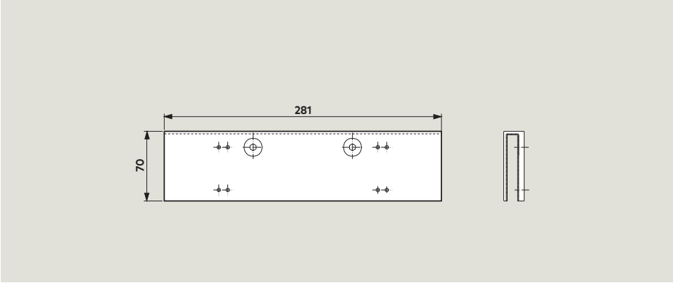
Glass door saddle plate for TS 92 For fixing the closer to toughened glass doors – No glass drilling or recessing required.
