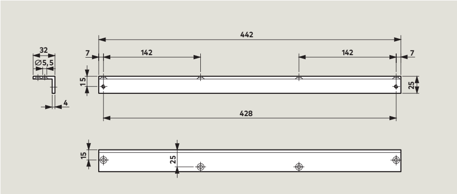
Angle bracket for G-N For push-side fixing of the slide channel to door frames with a deep reveal.
