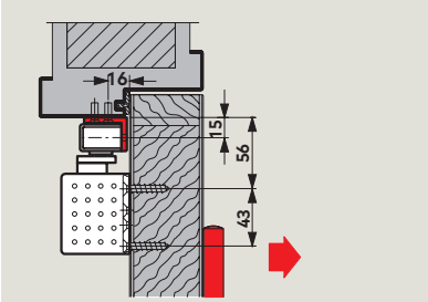
Angle bracket for G-N For push-side fixing of the slide channel to door frames with a deep reveal.
