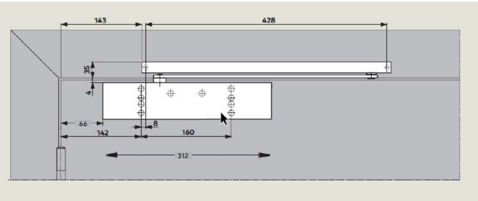
TS91/92 Softline or Square full covers Available in Silver, stainless steel, polished chrome, polished brass and coloured.
