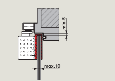
Glass door saddle plate for TS 92 For fixing the closer to toughened glass doors – No glass drilling or recessing required.
